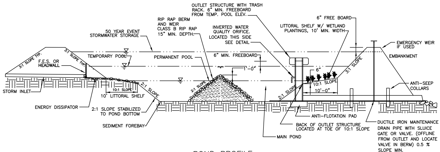
POND PROFILE
