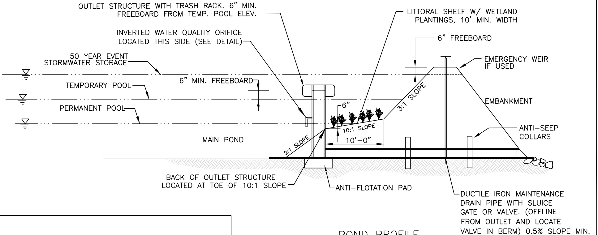
POND PROFILE
